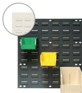
QLP-1819 18"L x 19"H Accepts all sizes of Ultra Bins. 175 lb. load capacity. (Bins sold separately)
