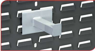
WS-HDS6 Heavy-Duty 6" Spike 65 lb. load capacity
